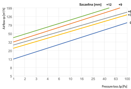
ASV160-ML - air supply
