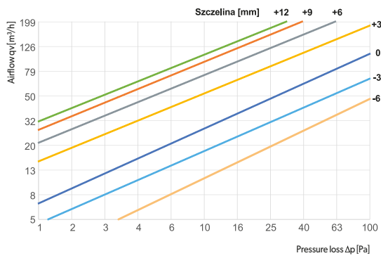
ASV150-ML - air supply
