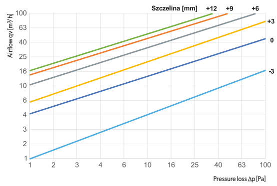
ASV100-ML - air exhaust
