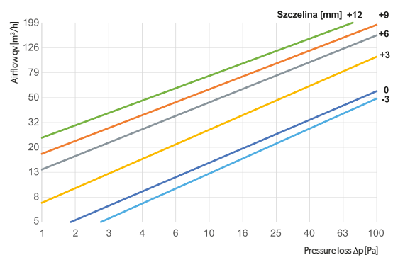
ASV125-ML - air exhaust
