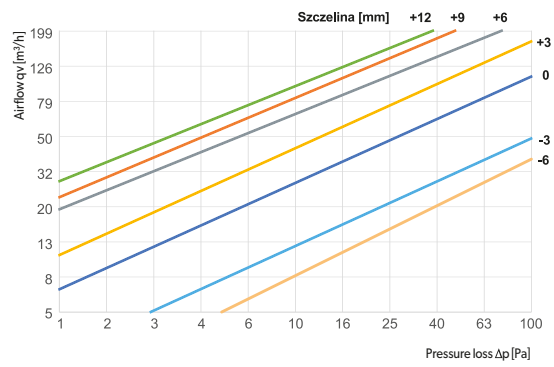
ASV150-ML - air exhaust
