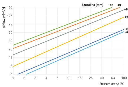
ASV125-ML - air supply
