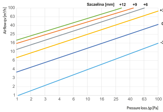
ASV100-ML - air supply
