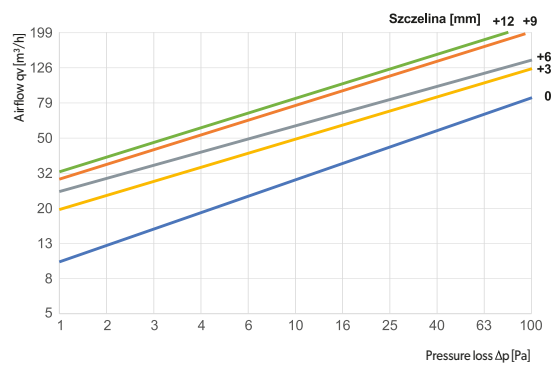
ASV160-ML - air exhaust
